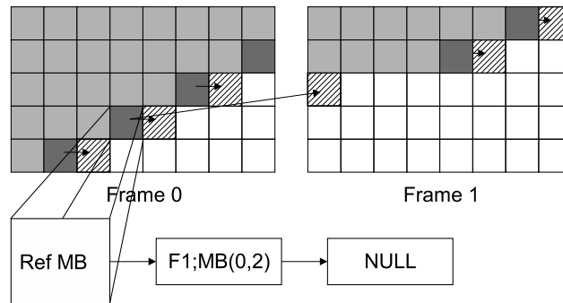
Fig. 6. Illustration of the 3D-Wave and the subscription mechanism.
