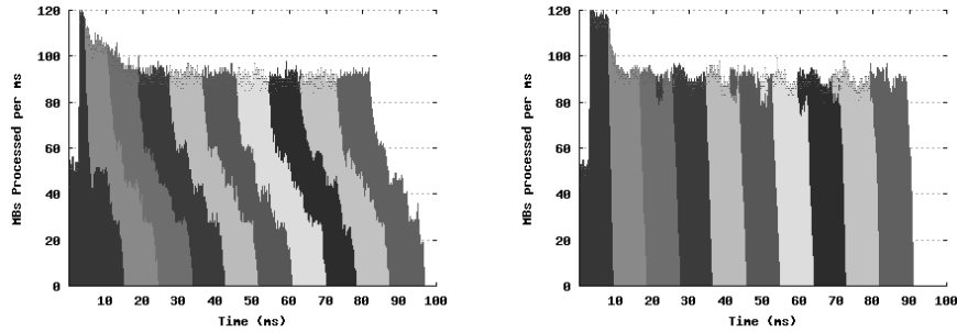
(a) Number of MBs processed per ms using frame scheduling and frames to which these MBs belong.
