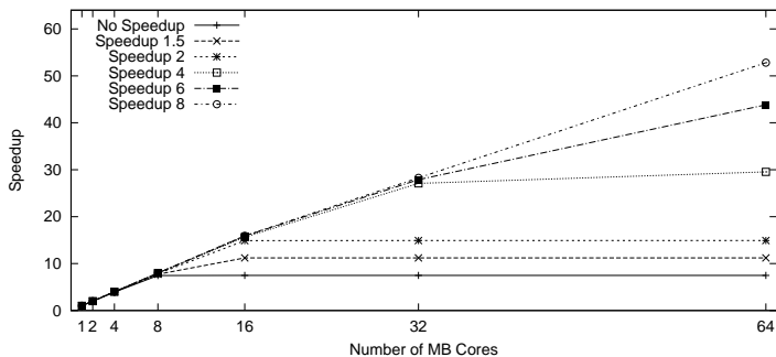
Fig. 14. Maximum scalability per CABAC processor and accelerators
