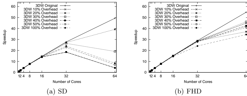
Fig. 13. TPL overhead effects on scalability for Rush Hour frames
