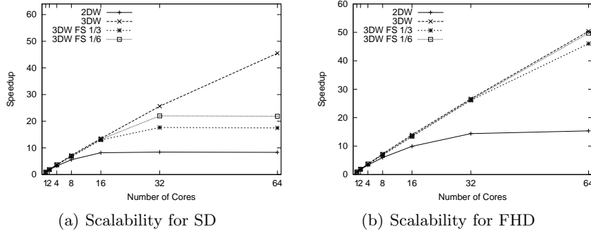
Fig. 9. Frame scheduling and priority scalability results of the Rush Hour 25-frame sequence
