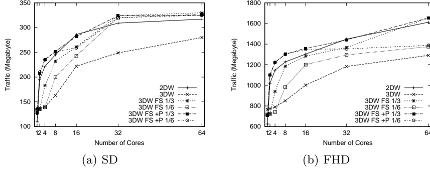
Fig. 10. Frame scheduling and priority data traffic results for Rush Hour sequence.
