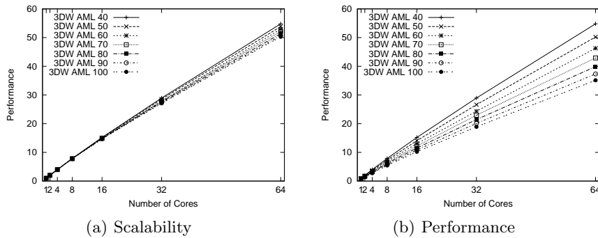
Fig. 11. Scalability and performance for different Average Memory Latency (AML) values, using the 25 frame Rush Hour FHD sequence. In the scalability graph the performance is relative to the execution on a single core, but with the same AML. In the performance graph all performances are relative to the execution on a single core with an AML of 40 cycles.
