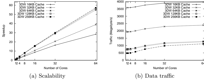
Fig. 12. Impact of the L1 cache size on performance and L1-L2 traffic for a 25 frame Rush Hour FHD sequence.
