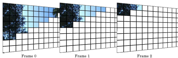
Fig. 2. 3D-Wave strategy: frames can be decoded in parallel because inter-frame dependencies have a limited spatial range.
